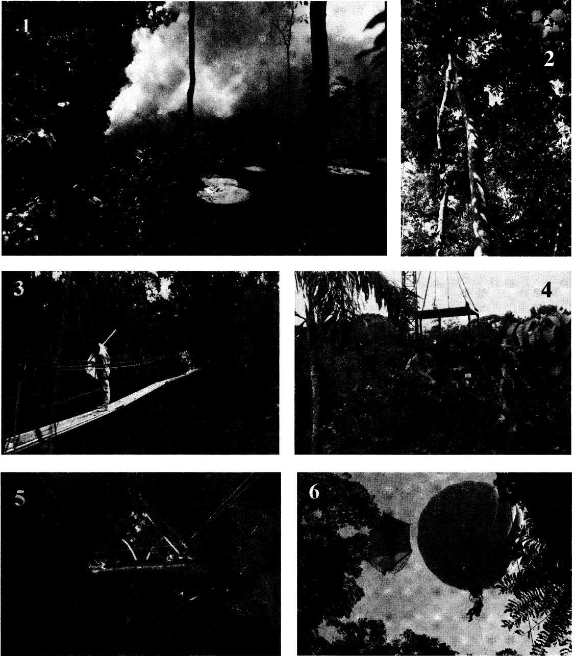
Fig. 2.1. Methods of canopy access and entomological techniques. 1. Mist-blowing in Australia (photo H. Setsumasa). 2. Beating the foliage with single-rope techniques in Papua New Guinea (photo Y. Basset). 3. Netting insects on a walkway in Sarawak (photo H. Setsumasa). 4. Observation of foliage with the canopy crane near Colon, Panama (photo M. Guerra). 5. Harvesting foliage samples with the canopy sledge, Cameroon (photo H. Setsumasa). 6. Surveying interception-flight traps with the treetop bubble, Gabon (photo H. Setsumasa).
